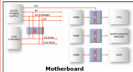
Motherboard
